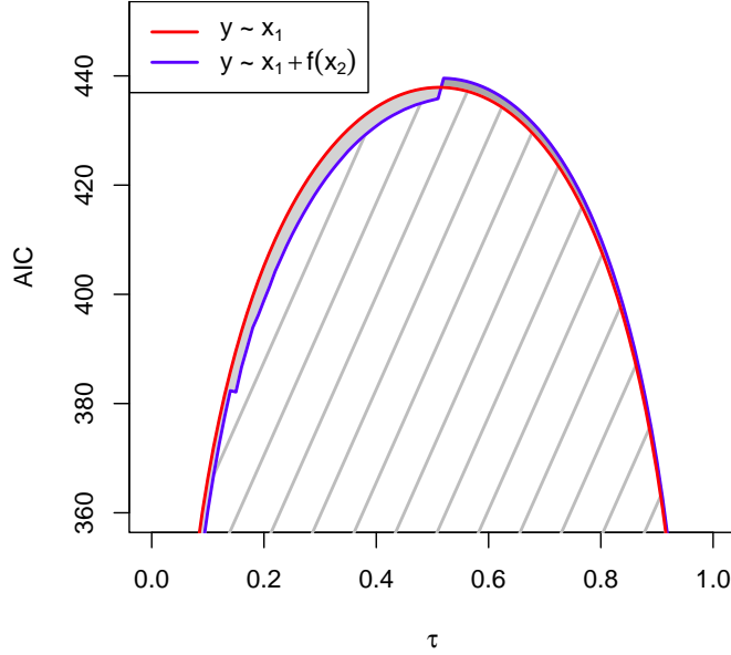
Figure 1: Differences between models as area between the criteria curves. This graphic is based on the exponential simulation design of Section 4, but with more extreme parameters and fewer observations.
