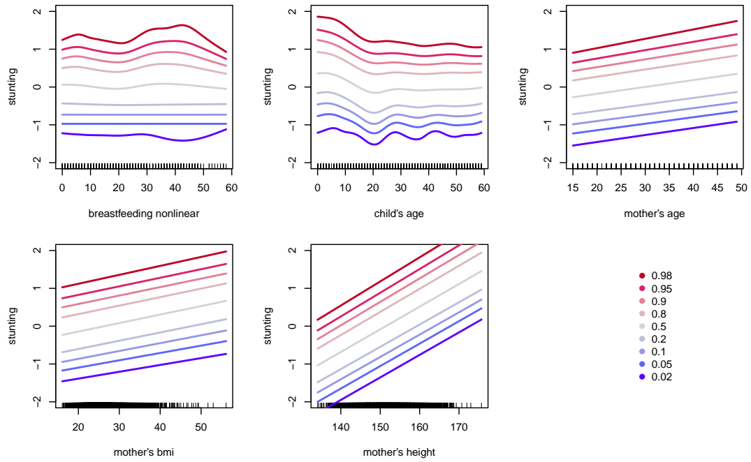
Figure 6: Estimated coefficients of metric covariates selected via scoring
