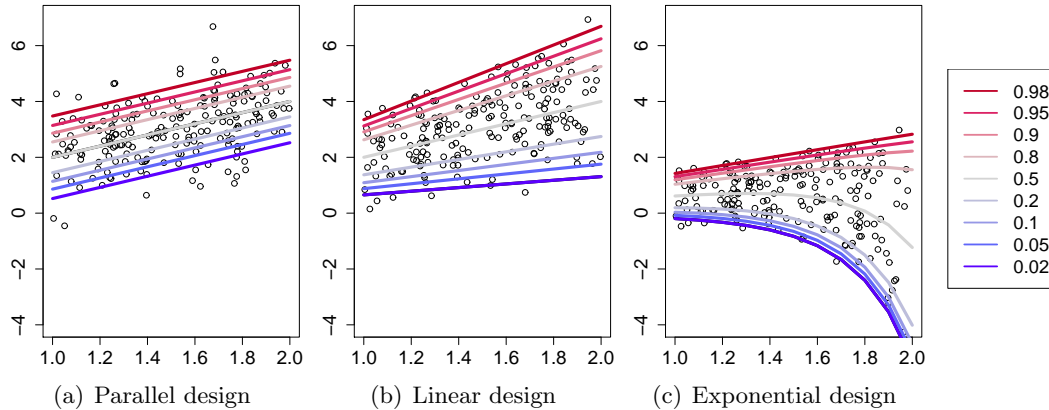
Figure 2: Simulation design for f_{2,\tau} in all three data settings.
