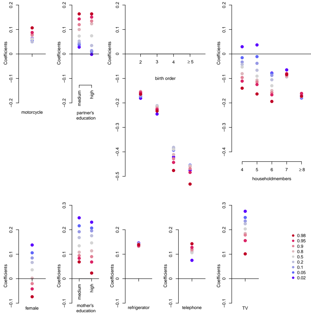
Figure 5: Estimated coefficients of categorical covariates selected via scoring
